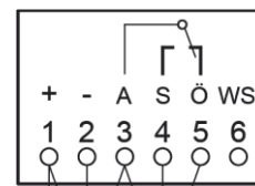
Rain detector RM/2 24V
