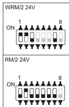
DIP switch setting
