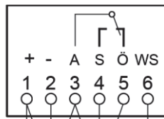
Wind-/ rain detector WRM/2 24V
