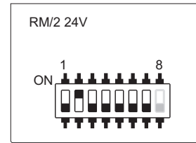
DIP switch setting
